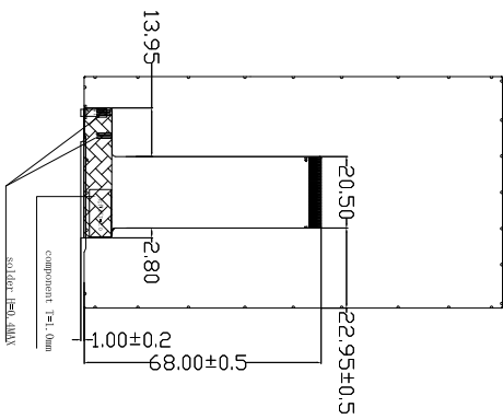
FPC bending shipping diagram
