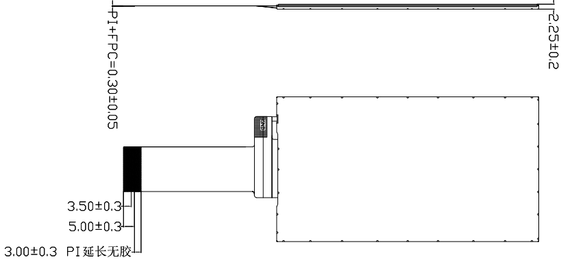
FPC bending shipping diagram
